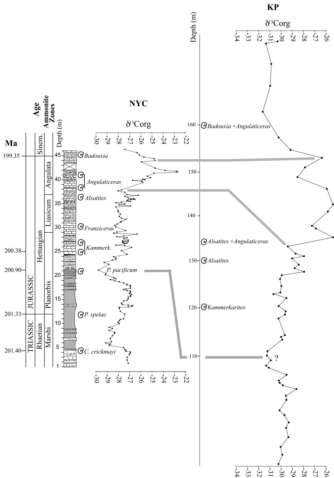
Figure 1. Ammonite biostratigraphical calibration of the organic carbon isotope curve at New York Canyon (NYC) Nevada USA, correlated with the Kennecott Point (KP) curve [Williford et al., 2007] recalibrated with the age diagnostic ammonites identified by Longridge et al. [2008]. U-Pb numerical ages are from Schaltegger et al. [2008] and Schoene et al. [2010].
