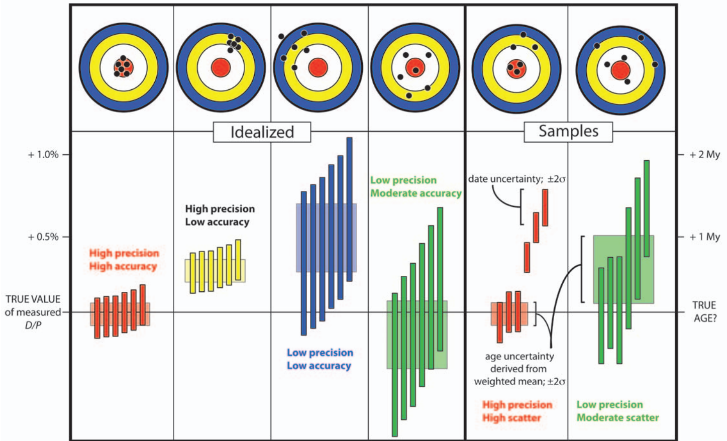
FIGURE 1 What is the difference between precision and accuracy? This schematic plot illustrates variably accurate and precise data sets. The top panel is a series of bull's-eye targets typical of those used to illustrate precision and accuracy. Below them are plots more typical of those used in geochronology studies, which show ratios or dates versus analysis number. The colored bars represent single analyses, and the height of the bar reflects the 2-sigma uncertainty for that analysis. The y-axis is in percent of the true daughter to parent ratio ( D/P ) on the left and in millions of years on the right. The partly transparent boxes behind groups of analyses represent a weighted-mean value for that group, with the box height equivalent to \pm 2 -sigma uncertainty.
