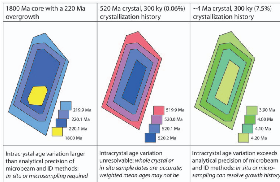
FIGURE 2 Precision versus accuracy in minerals with complex growth histories.
